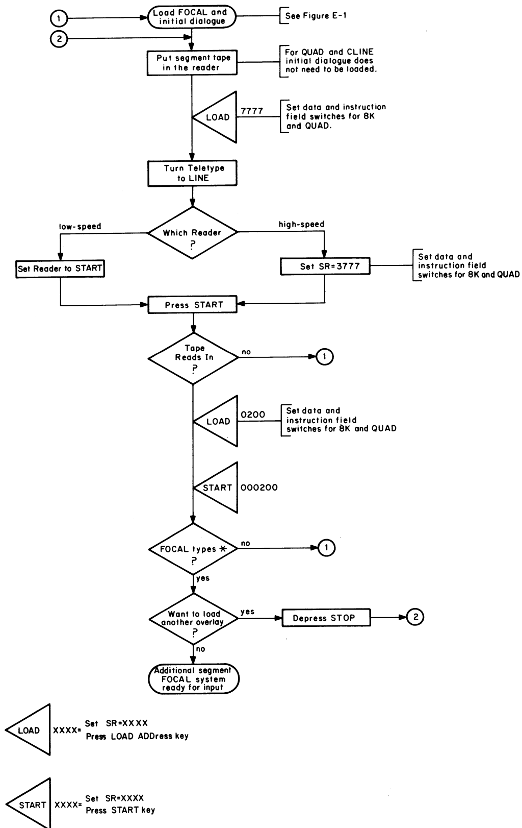
Figure E-3 Additional System Segments Loading Procedure
